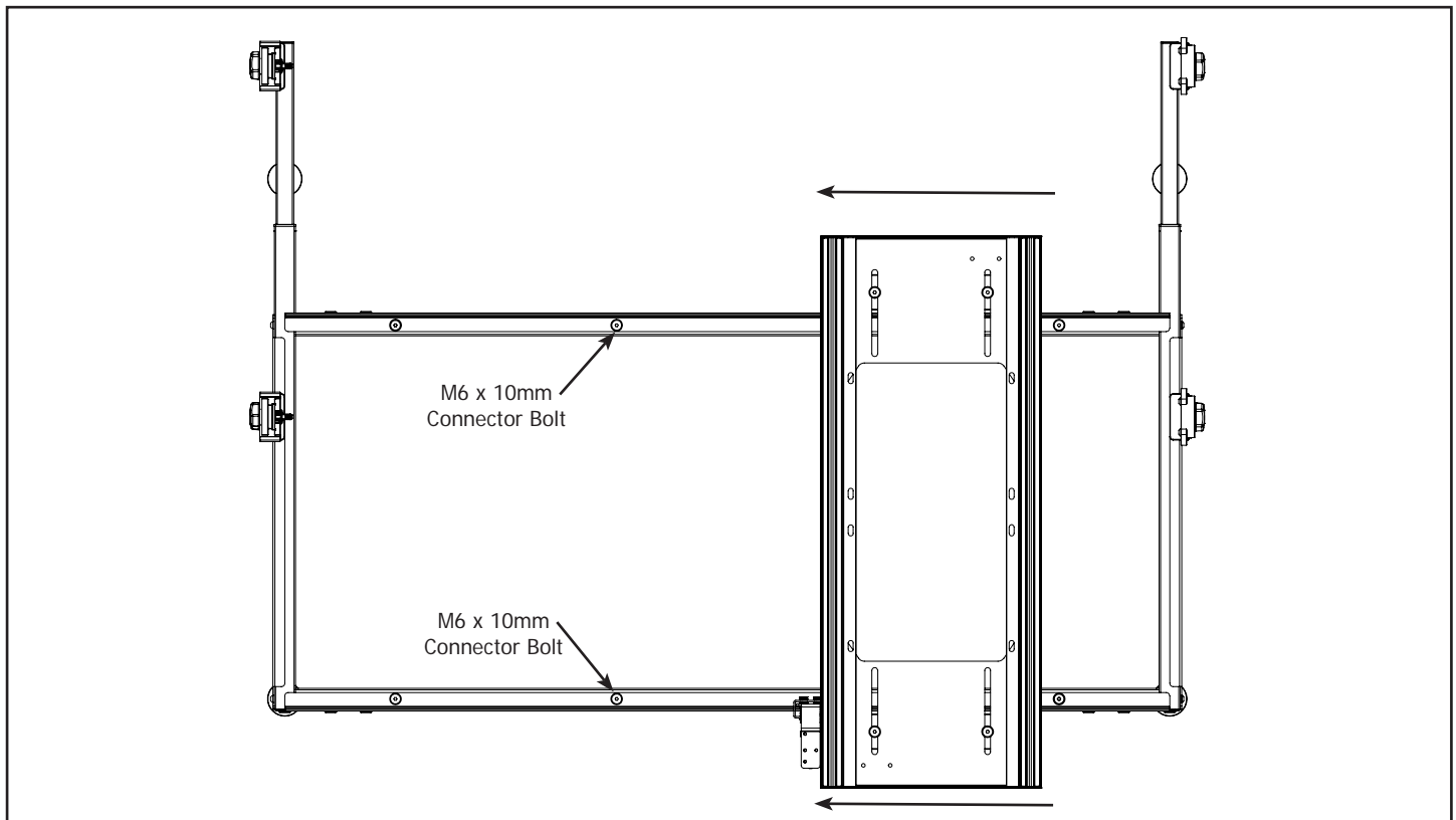
5-5 Align the track by slowly moving the Carriage along the track, working from one end to the other, tightening each of the back (4) M6 x 10mm Connector Bolts as you go.
