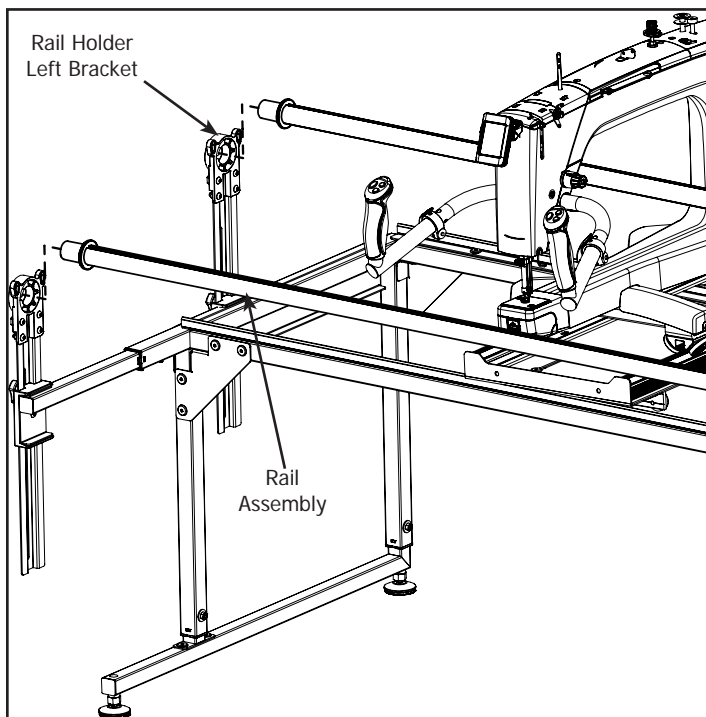
15-3 Remove the front Rail Assembly from the Rail Holder Left Bracket. Slide the remaining Rail Assembly out of the Rail Holder Left Bracket and out through the throat of the sewing machine.
