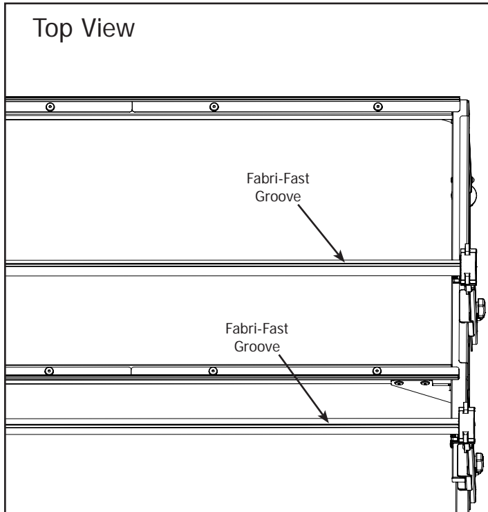
15-1 Rotate the Rail Assemblies to have the Fabri-Fast groove is faced up.
