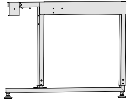
Right Leg (1) (QZF-09-13060)
