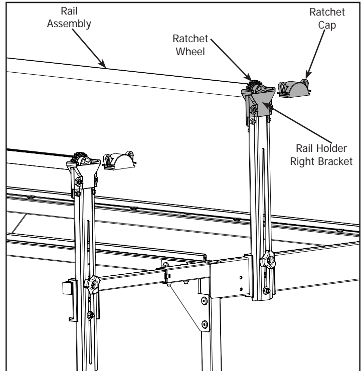
15-2 Slide the Ratchet Caps off of the Rail Holder Right Brackets.
