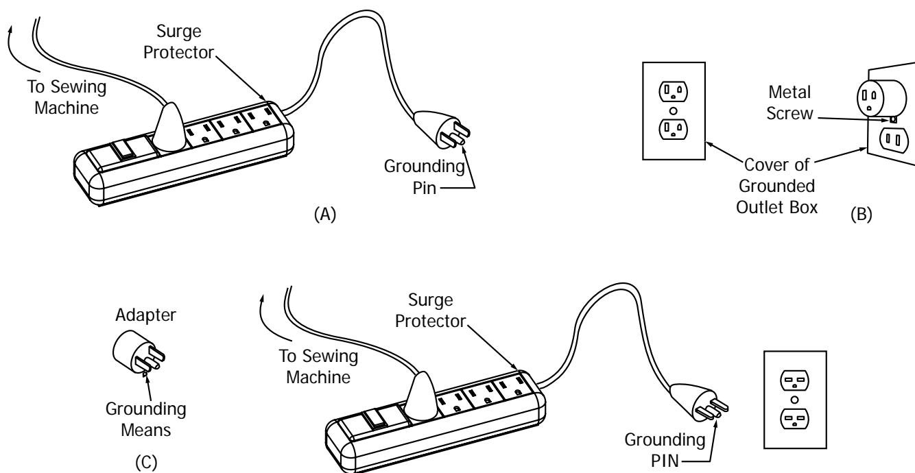
Grounding Methods
