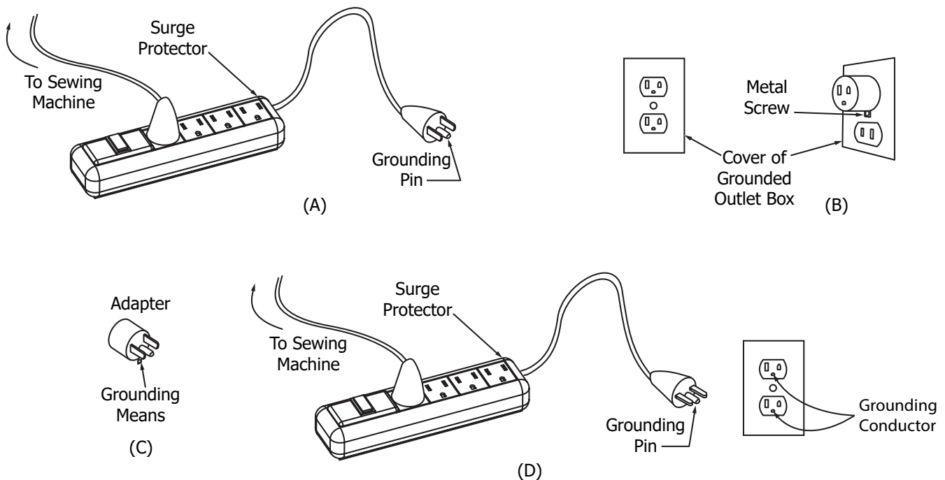
Grounding Methods
