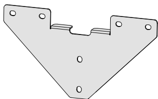
Middle Leg Brace (2) (QZH-04-12060)
