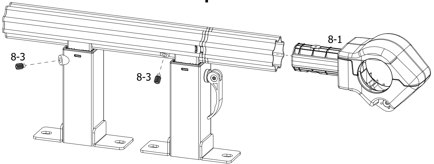
DOM Side Rail Tower with Ratcheted Rail Plastics Assembly QEF-09-16570
