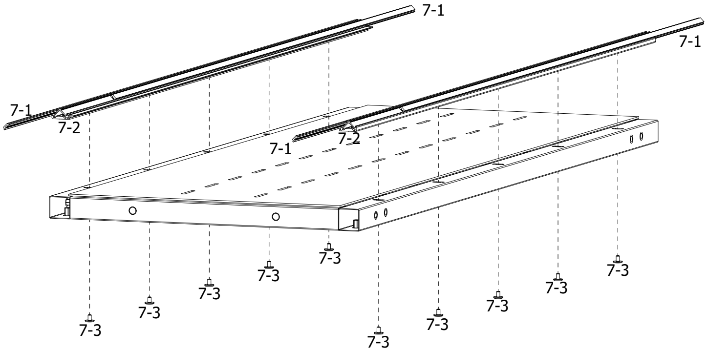
5ft Table Assembly QEF-09-16576
