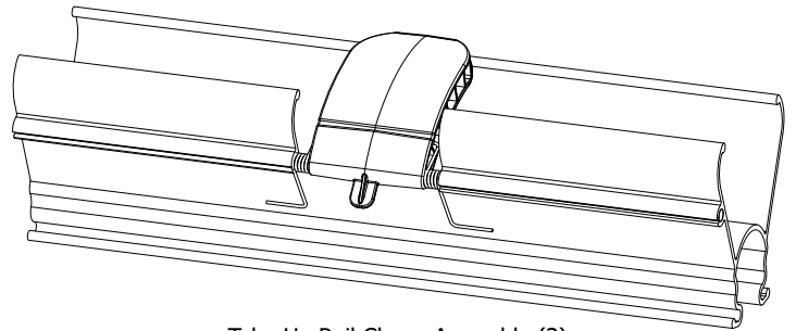
Take-Up Rail Clamp Assembly (3) QEF-09-16566
