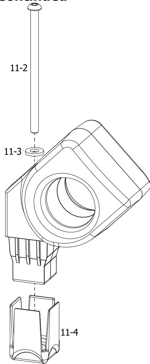
Take-Up Rail Holder Floating Rail Plastics Subassembly QEF-09-16581
