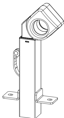
Take-Up Rail Tower - Left (1) QEF-09-16580
