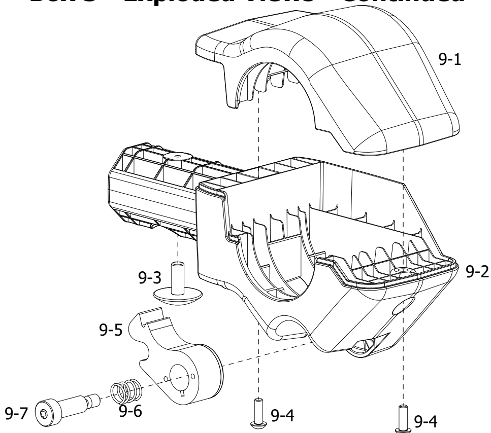
Front Corner Assembly - Ratchet Side - DOM Version QEF-09-16571
