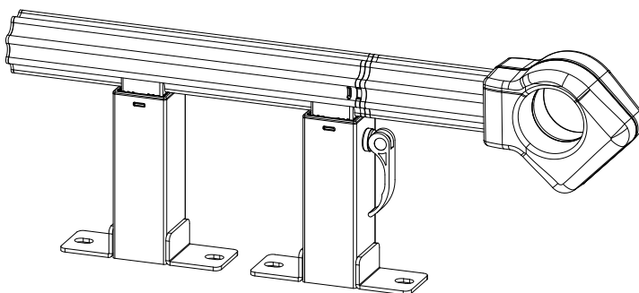
DOM Side Rail Tower with Floating Rail Plastics Assembly (1) QEF-09-16531
