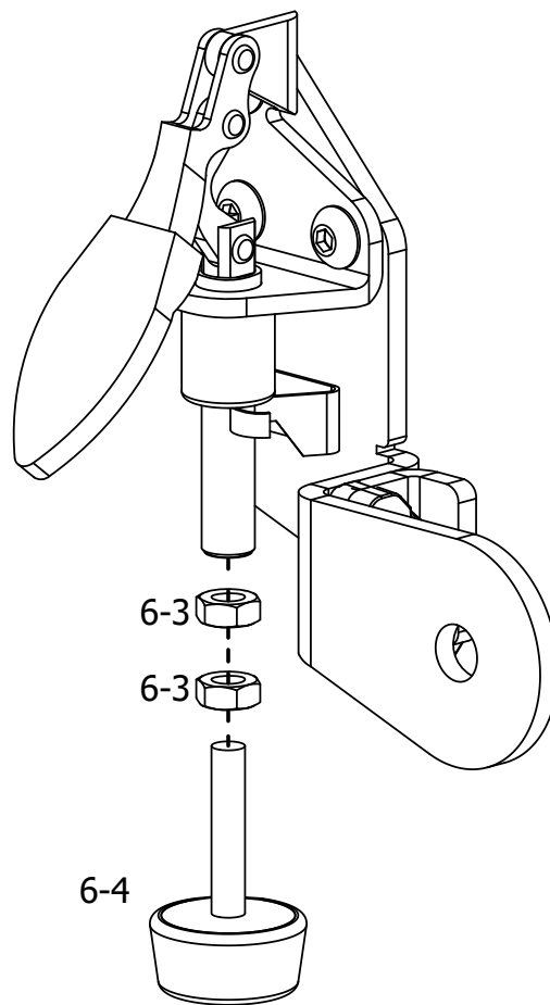
Channel Lock ACC-09-13057
