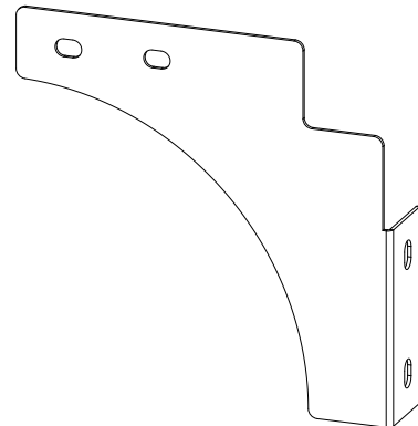
Corner Brace B (2) QEF-04-15544
