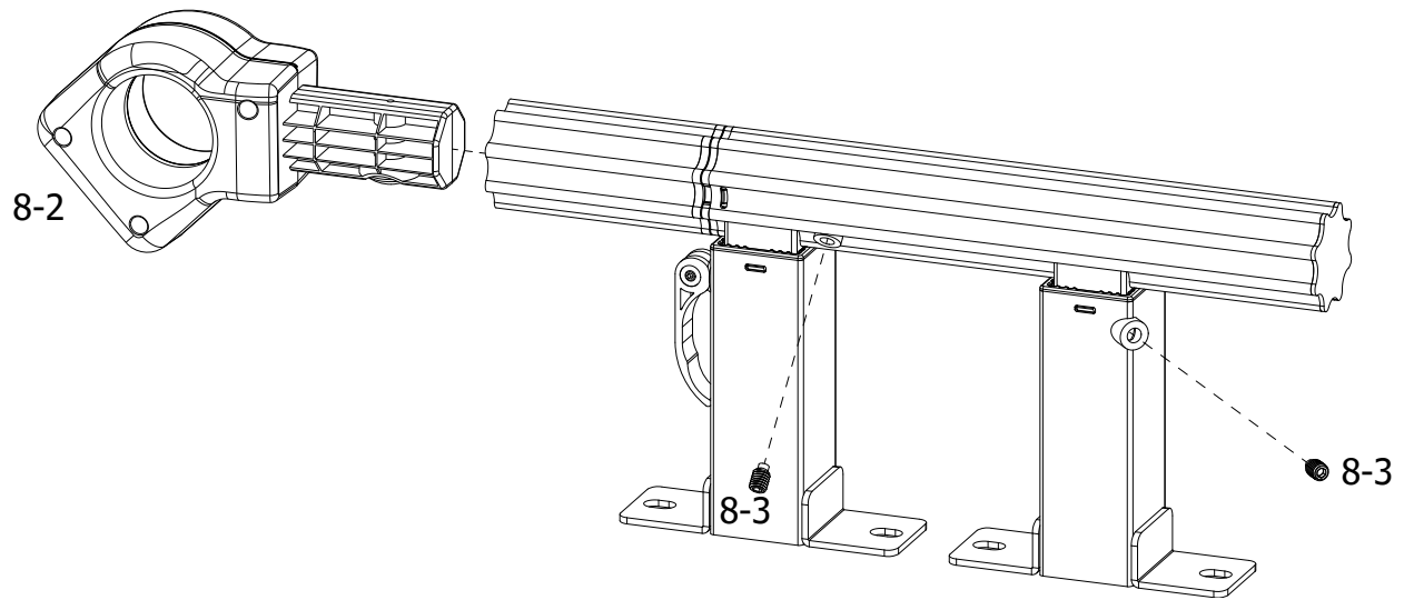
DOM Side Rail Tower with Floating Rail Plastics Assembly QEF-09-16531
