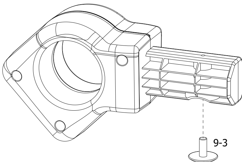
DOM Side Rail Tower with Floating Rail Plastics Assembly QEF-09-16531
