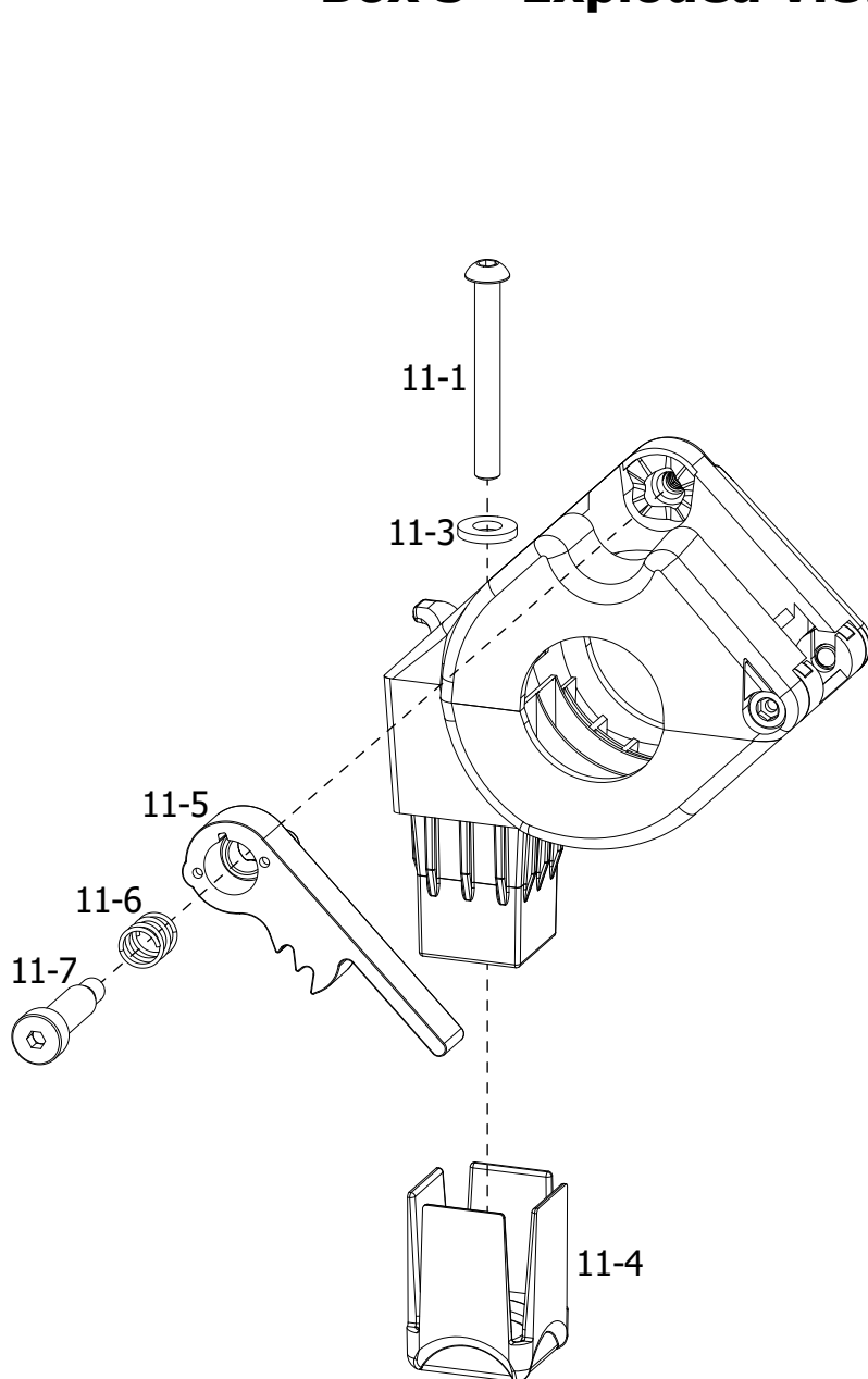
Take-Up Rail Holder Ratcheting Plastics Subassembly QEF-09-16543
