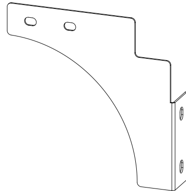
Corner Brace B (2) QEF-04-15544
