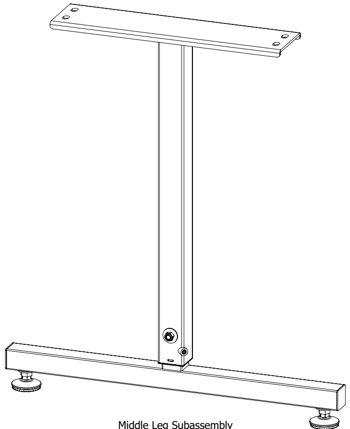
Middle Leg Subassembly QEF-09-17102
