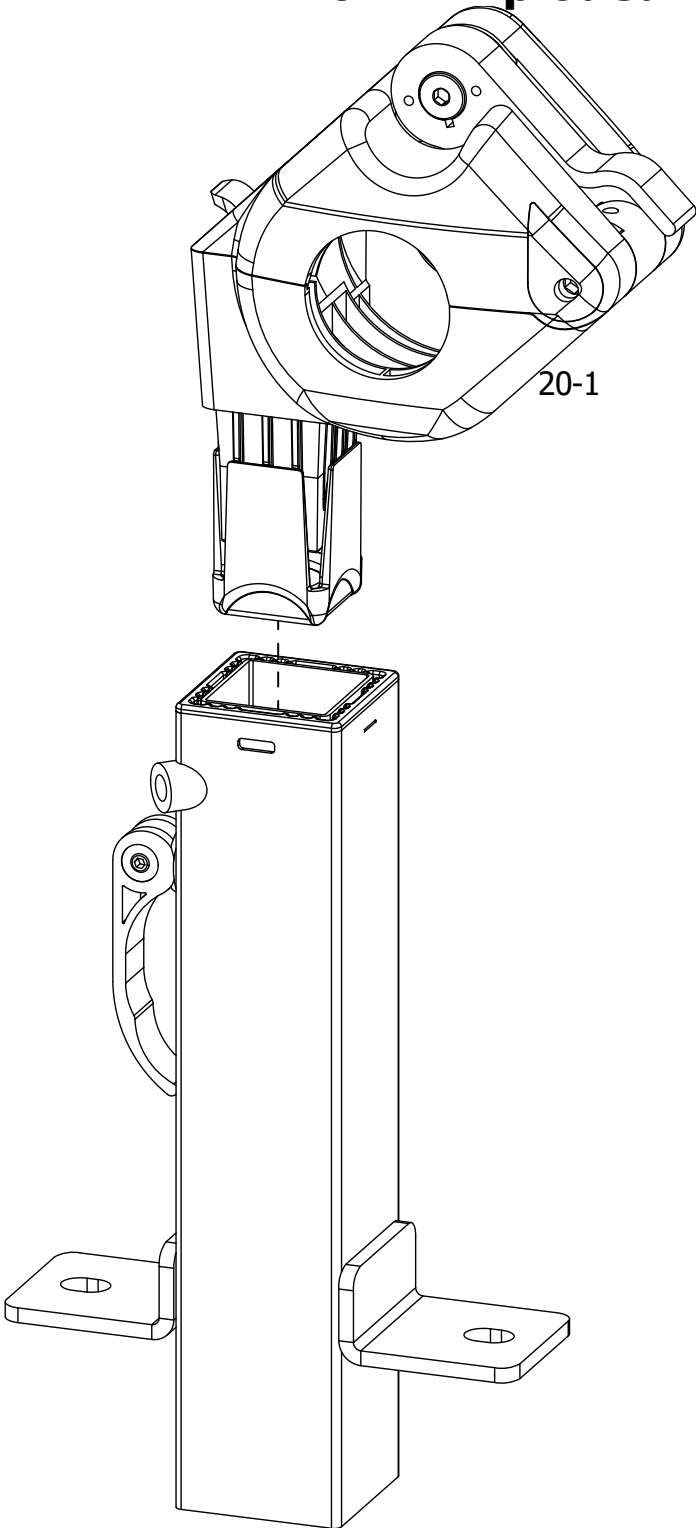
Right Take-Up Rail Tower - Elite Frame QEF-09-17034
