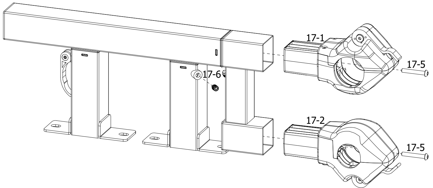
Square Side Rail Assembly - Right QEF-09-17044
