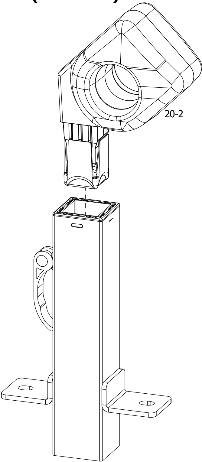
Left Take-Up Rail Tower - Elite Frame QEF-09-17030
