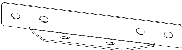
Middle Table Brace (2) QEF-04-15545
