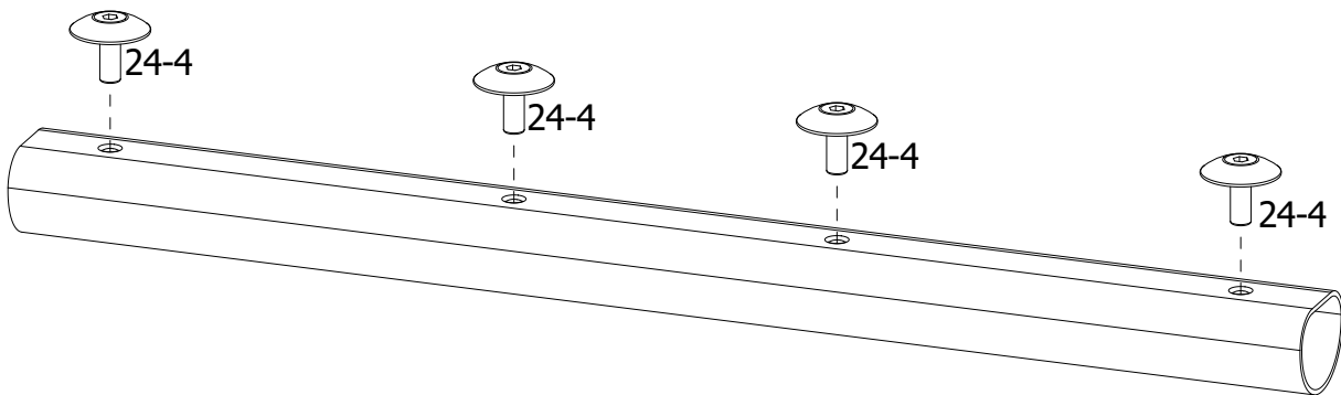
Rail Coupler Assembly CNT-09-11865
