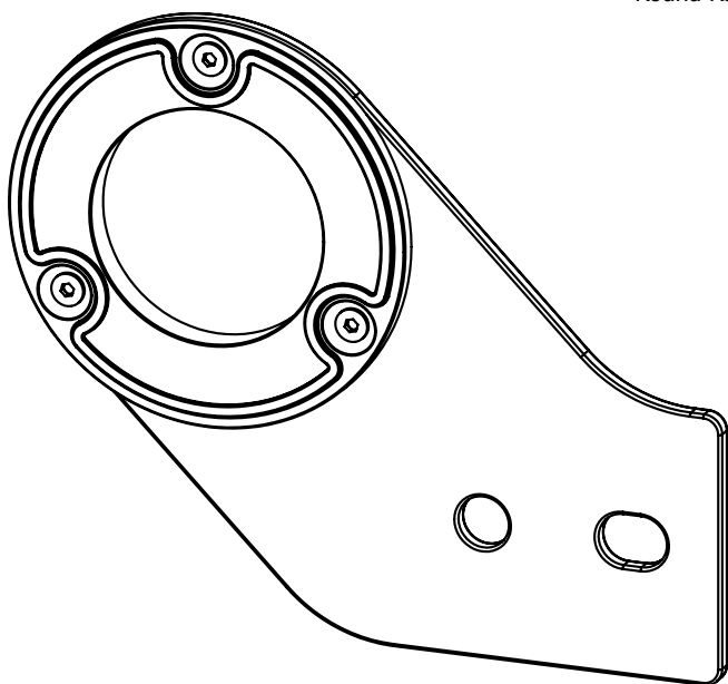
Accessory Rail Metal Bracket Assembly - Left (1) QEF-09-17189
