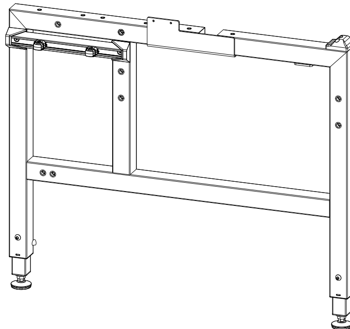
Right Side Leg Assembly (1) QEF-09-16563
