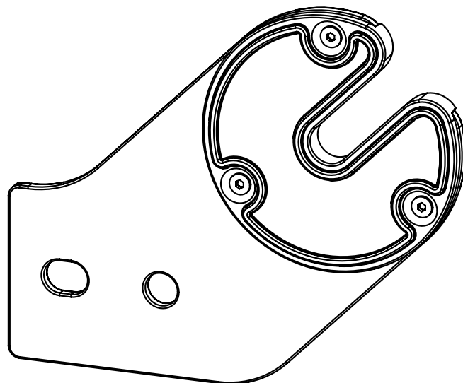
Accessory Rail Metal Bracket Assembly - Right (1) QEF-09-17188
