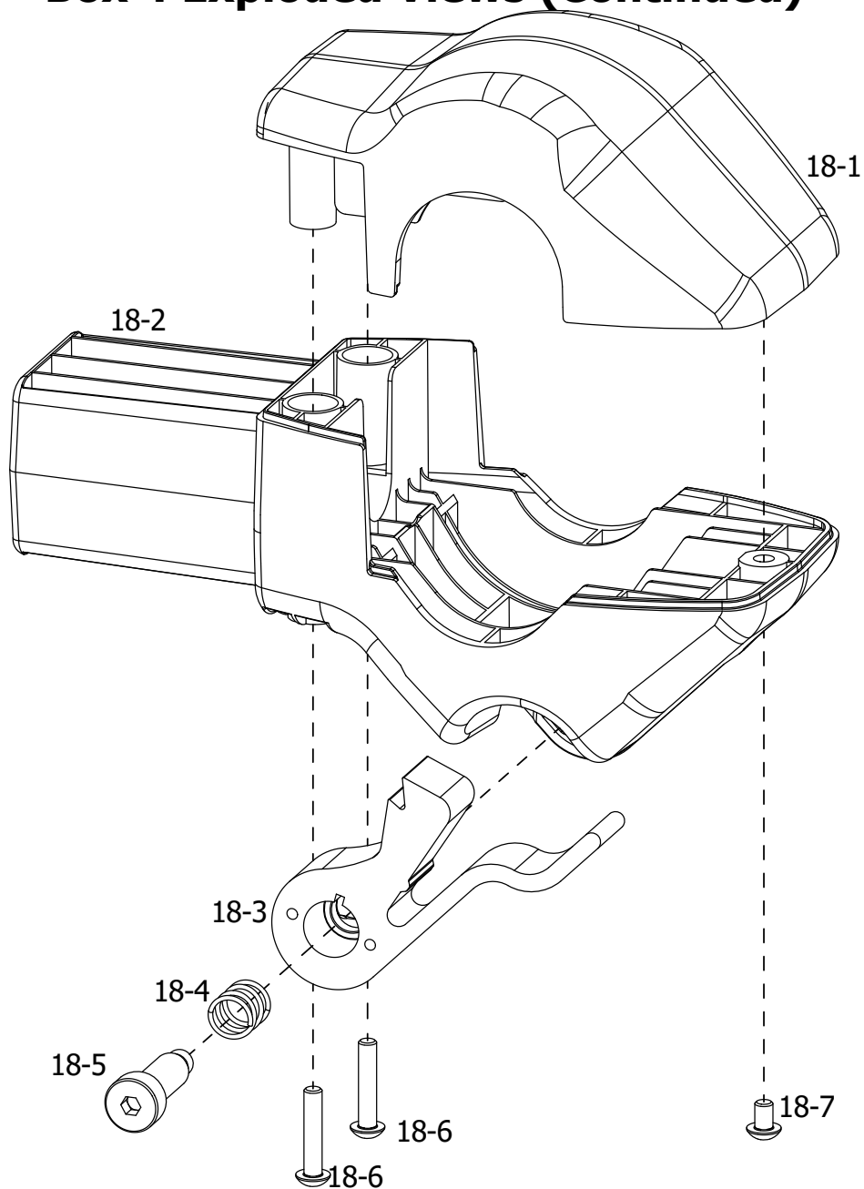
Quilt Top Rail Holder Assembly - Ratchet Side QEF-09-17045
