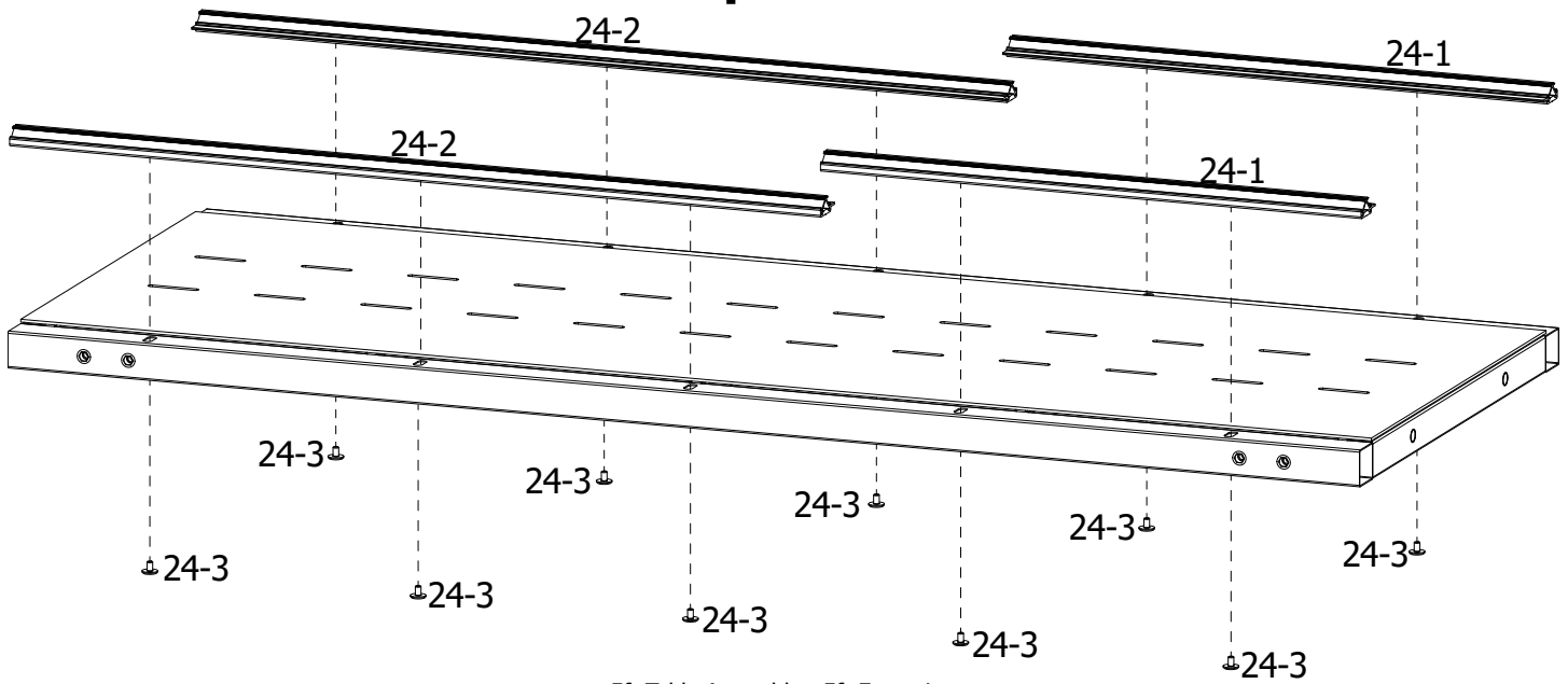
5ft Table Assembly - 5ft Extension QEF-09-17087
