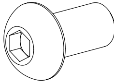
SBHCS M8 X 16mm (16) HDW-03-10951
