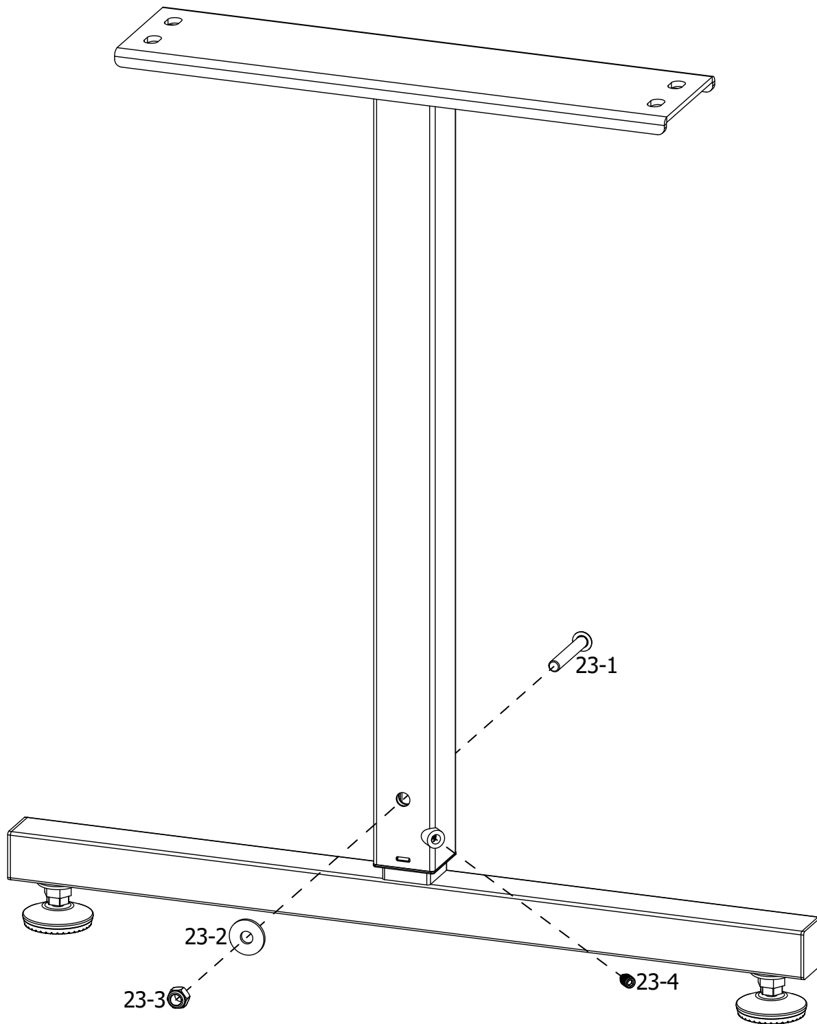
Middle Leg Subassembly QEF-09-17102
