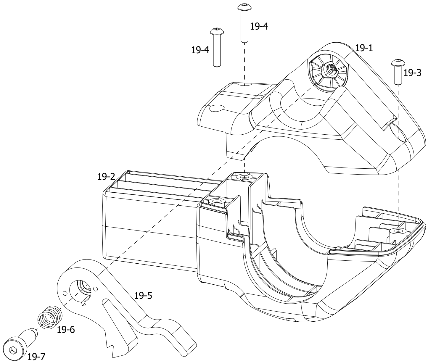
Quilt Back Rail Holder Assembly - Ratchet Side QEF-09-17050
