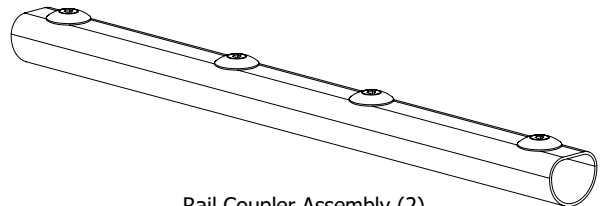
Rail Coupler Assembly (2) CNT-09-11865
