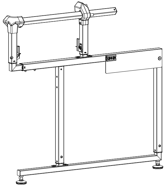
Right Leg Assembly (1) (QZH-09-14890)
