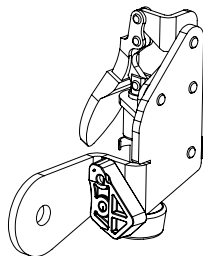
Sewing Machine Channel Lock (1) (ACC-09-13057)
