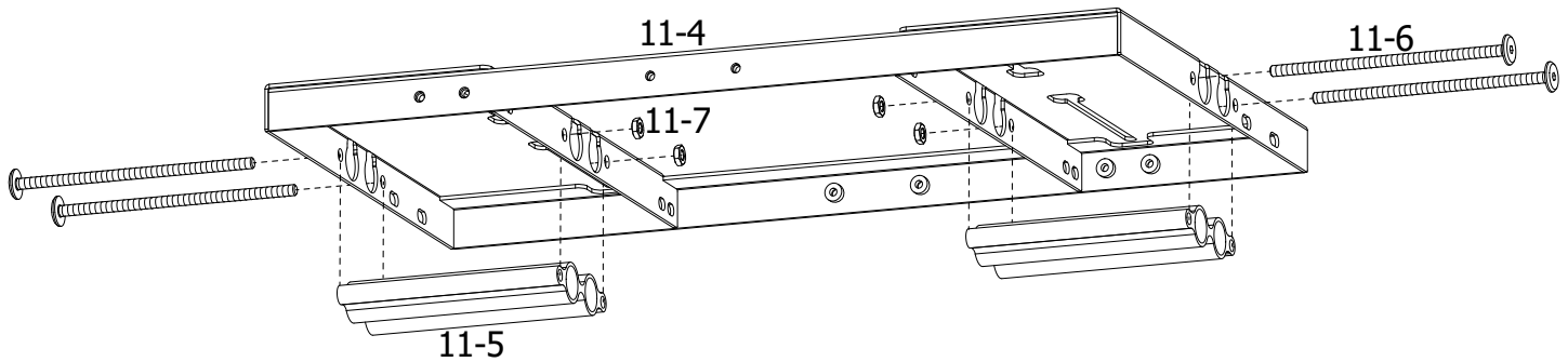
Top Plate with Guides Assembly QTT-09-14847
