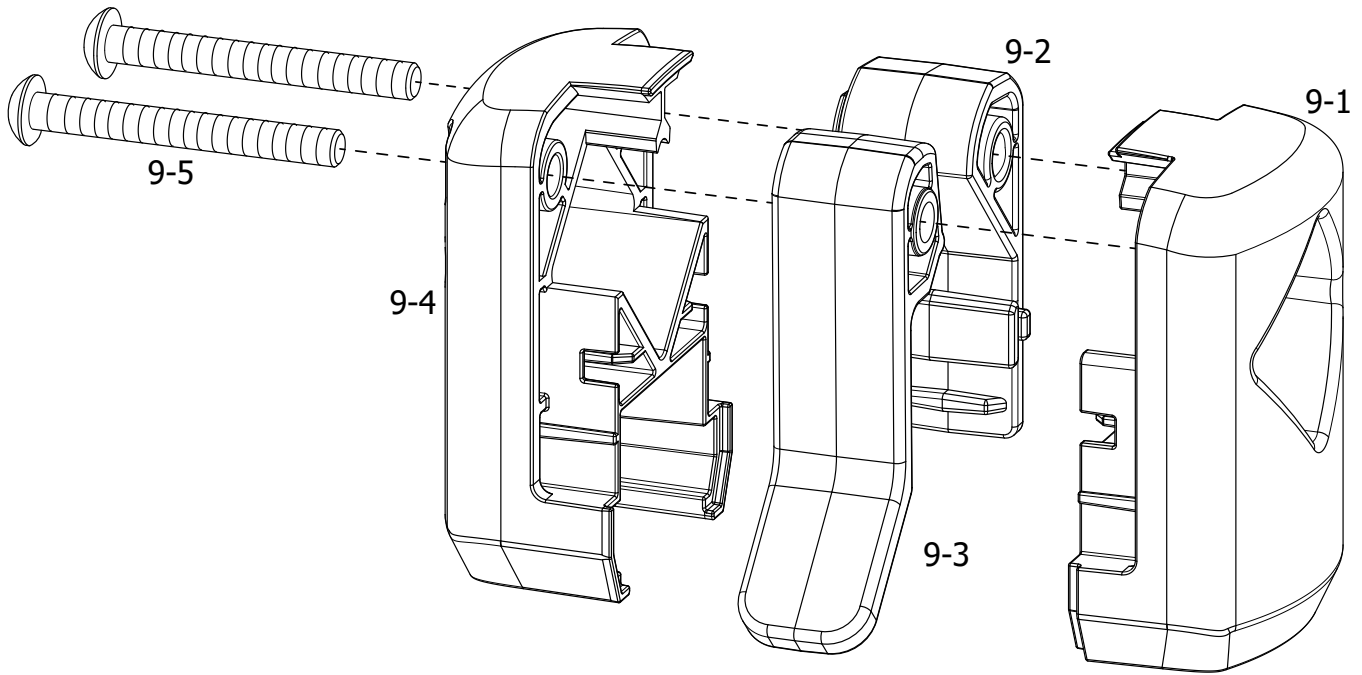
Rail Guide Assembly Right QTT-09-14862
