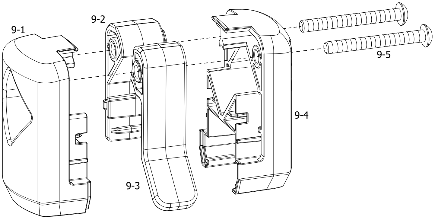
Rail Guide Assembly Left QTT-09-14833
