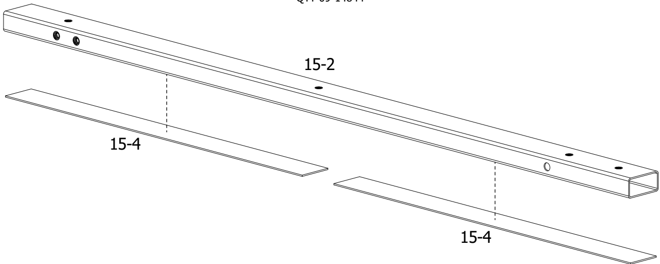
Long Cross Support QTT-09-14845
