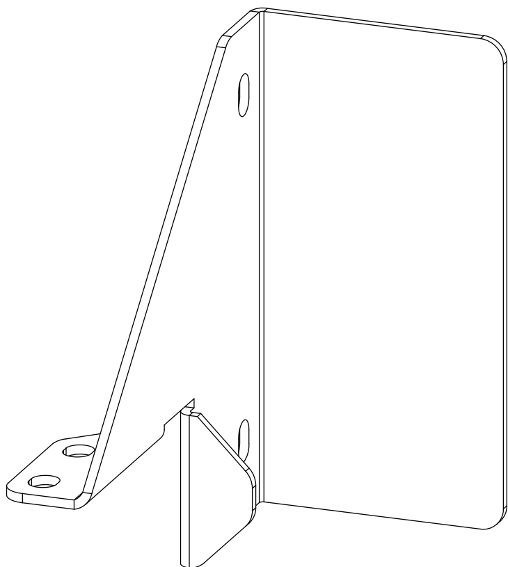
Back Left Brace (1) QTT-04-14822
