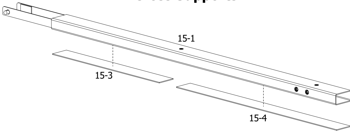
Short Cross Support QTT-09-14844
