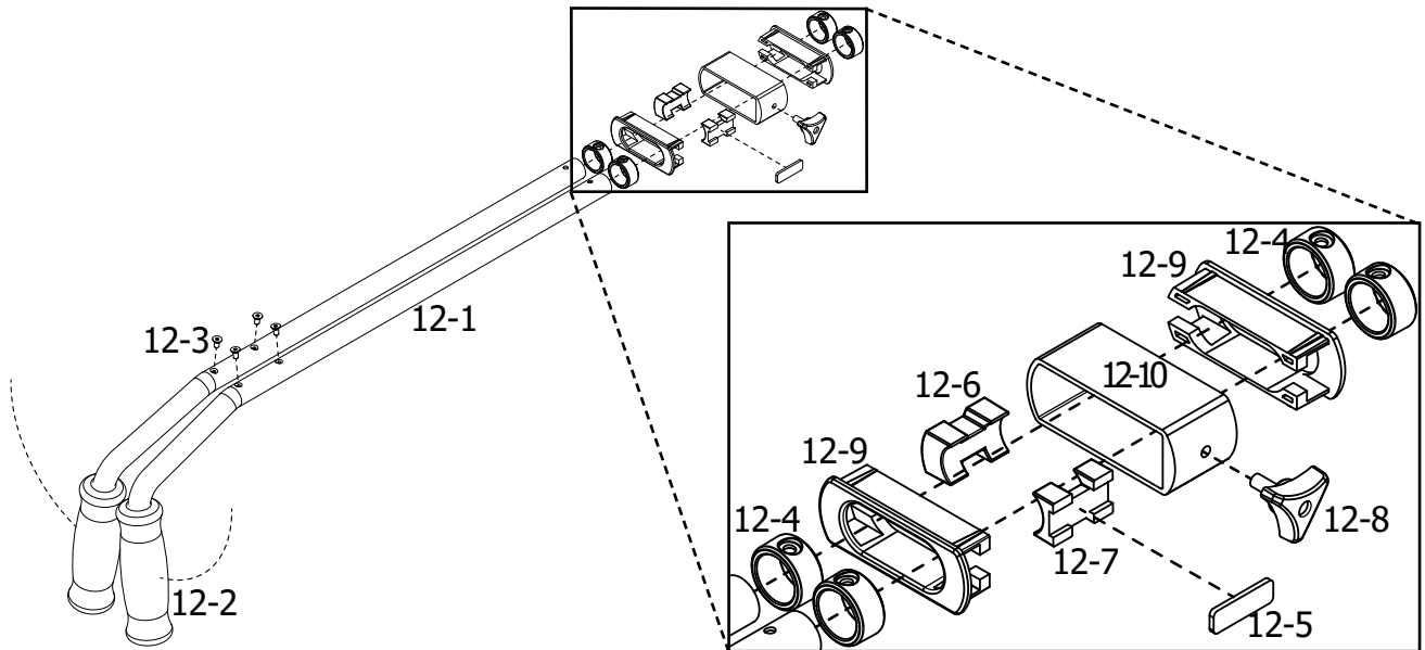
Handle Clamp Assembly and Handles QTT-09-14849
