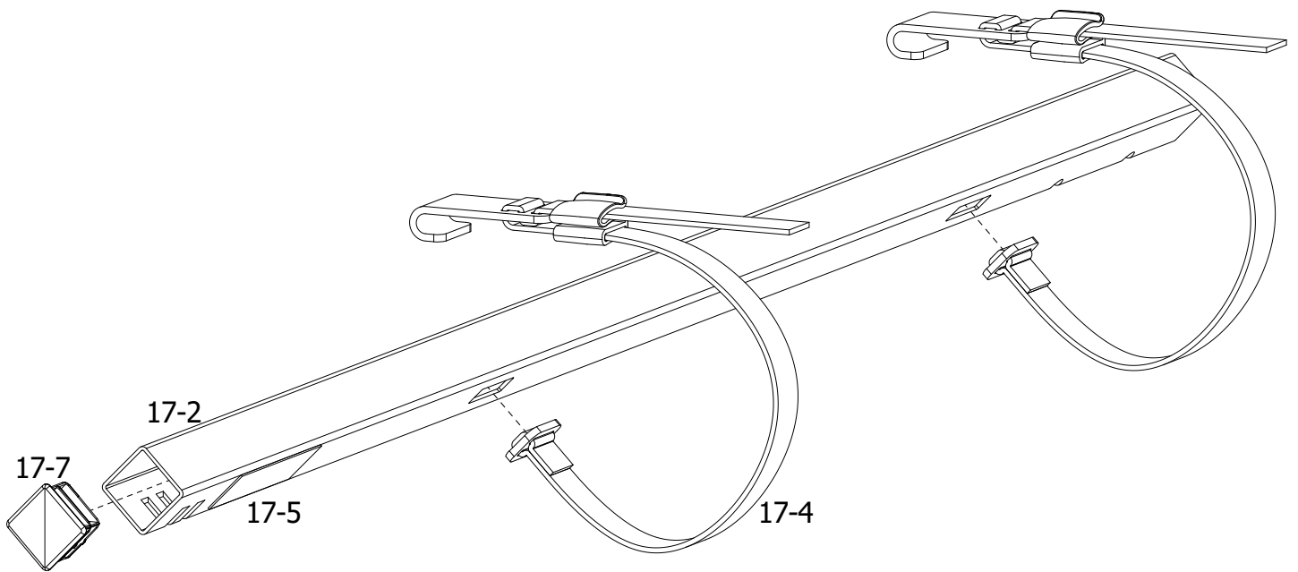
Long Take Up Rail QTT-09-14839
